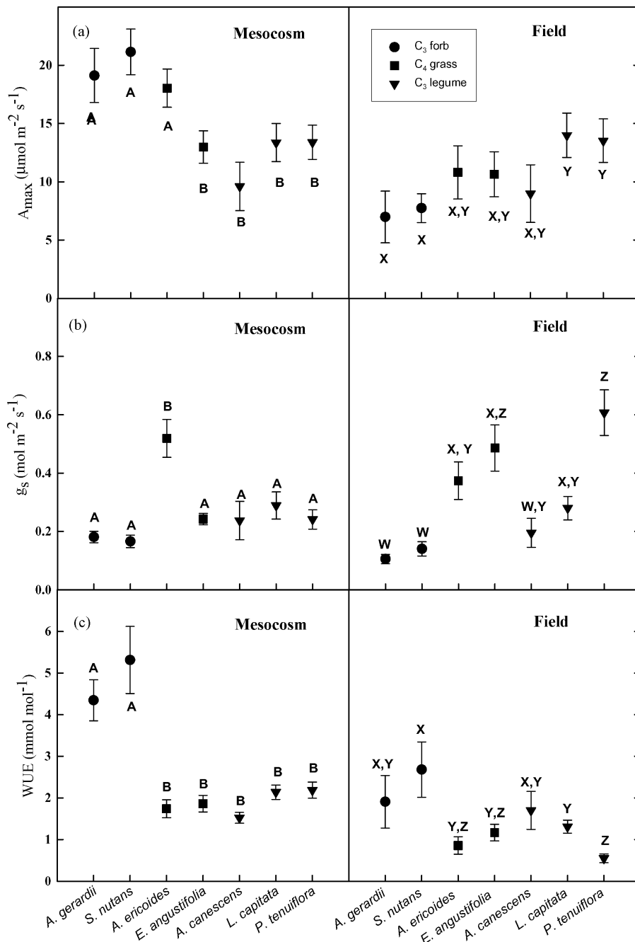
Fig. 2. Mean species response ( \pm 1 S.E.) for (a) \text{CO}_2 assimilation rate ( A_{max} ) at the ambient atmospheric \text{CO}_2 concentration ( \sim 370 \mu\text{mol mol}^{-1} ), (b) stomatal conductance to water ( g_s ) and (c) water-use efficiency (WUE). Species are arranged by their respective functional group for both the mesocosm and field locations. Points with varying letters indicate a significant difference ( P < 0.05 ) using Tukey's HSD.
