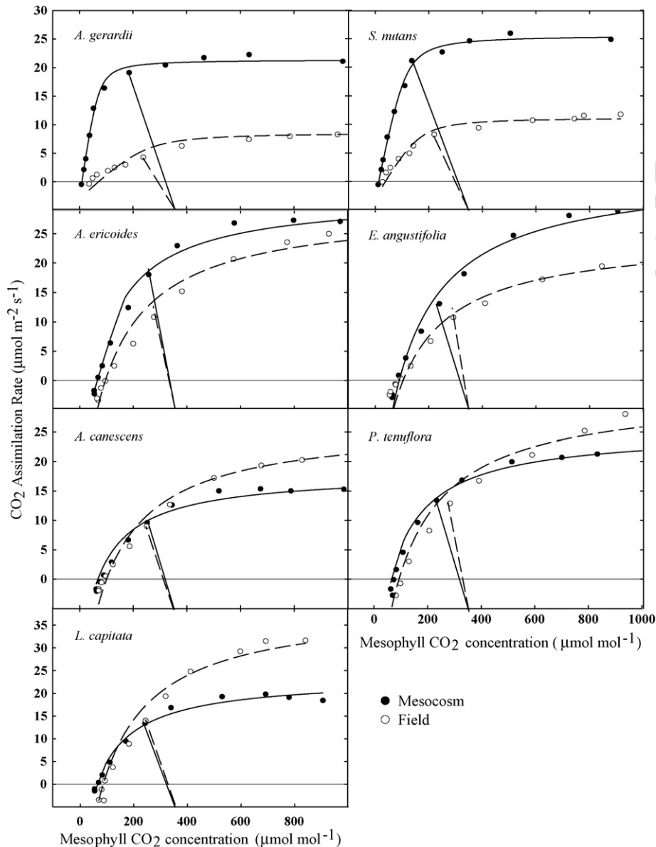
Fig. 4. Representative A:C_i fit for each species separately. A significant ( P=0.0072 , nDF=6 DF=89 ) species \times location relationship exists for the supply function. Each panel illustrates the CO 2 supply function from C_a ( 370 \mu\text{mol mol}^{-1} ) to the particular C_i associated with that measurement. Species are displayed separately with the solid line expressing the supply function for the mesocosm, and the dashed line for the field.
